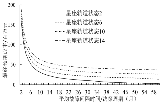
图 1 卫星平均故障间隔时间的增加对维护总成本的影响 Fig. 1 The influence of the increase of the mean time between failure of satellites on the total maintenance cost
