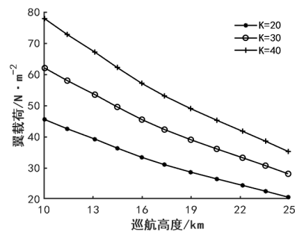
图2 翼载荷与飞行高度和升阻比的关系 Fig. 2 Relationship between wing load and cruising altitude and lift-drag ratio
