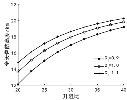
图1 全天巡航高度与升力系数和升阻比的关系 Fig. 1 Relationship between all-day cruising altitude and lift coefficient and lift-drag ratio
