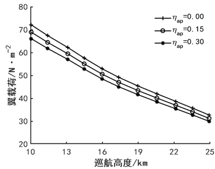
图 4 翼载荷与巡航高度和 \eta_{ap} 的关系 Fig. 4 Relationship between wing load and cruising altitude and \eta_{ap}
