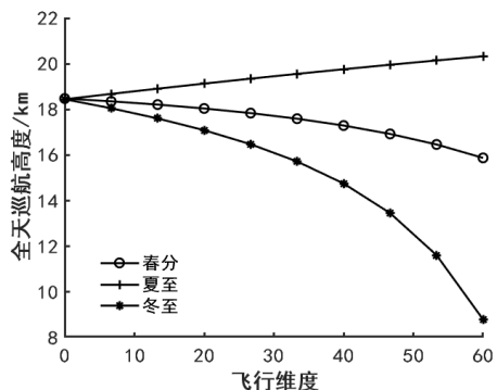
图 5 全天巡航高度与飞行纬度和飞行季节的关系 Fig. 5 Relationship between all-day cruising altitude and flight latitude and season
