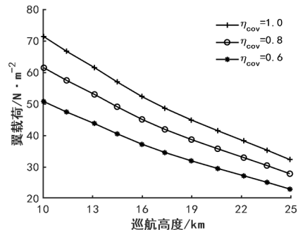
图8 翼载荷与巡航高度和 \eta_{cov} 的关系 Fig. 8 Relationship between wing load and cruising altitude and \eta_{cov}
